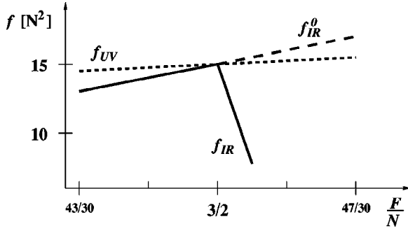
FIG. 1. Plot of f_{UV} and f_{IR} in units of N^2 as functions of F/N . We have taken the large- N and -F limit and show only the neighborhood of the interesting point F/N = 3/2 . For F/N < 3/2 one sees that f_{IR} < f_{UV} , at F/N = 3/2 the two f 's touch, and for F/N > 3/2 we again find f_{IR} < f_{UV} , but only after taking into account the interactions. For comparison we also show f_{IR}^0 , the expression for f_{IR} with no interactions included.
